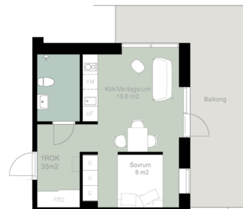
Lägenhet 6-1103, 6-1106, 6-1203, 6-1206 7-1103, 7-1106, 7-1203, 7-1206 8-1103, 8-1106, 8-1203, 8-1206
